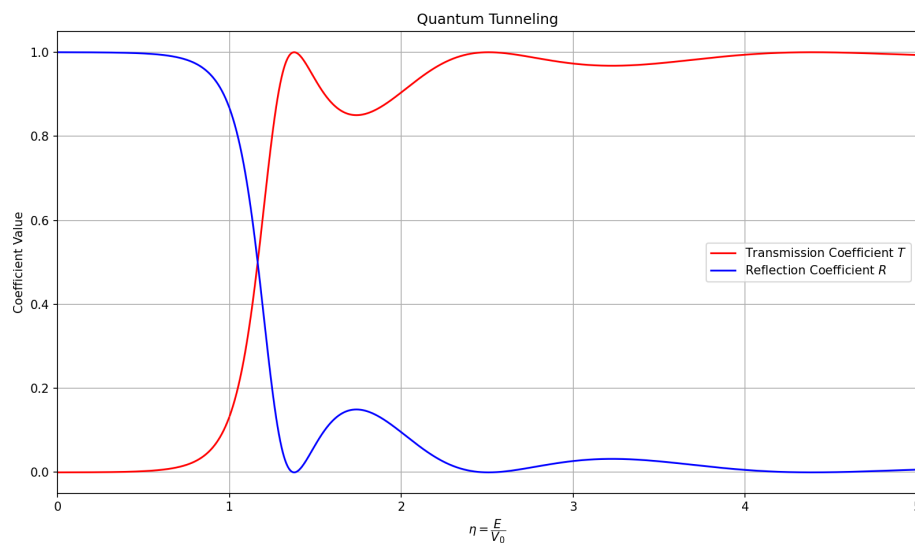
Figure 1: Quantum tunneling: Transmission and Reflection Coefficients vs \eta
